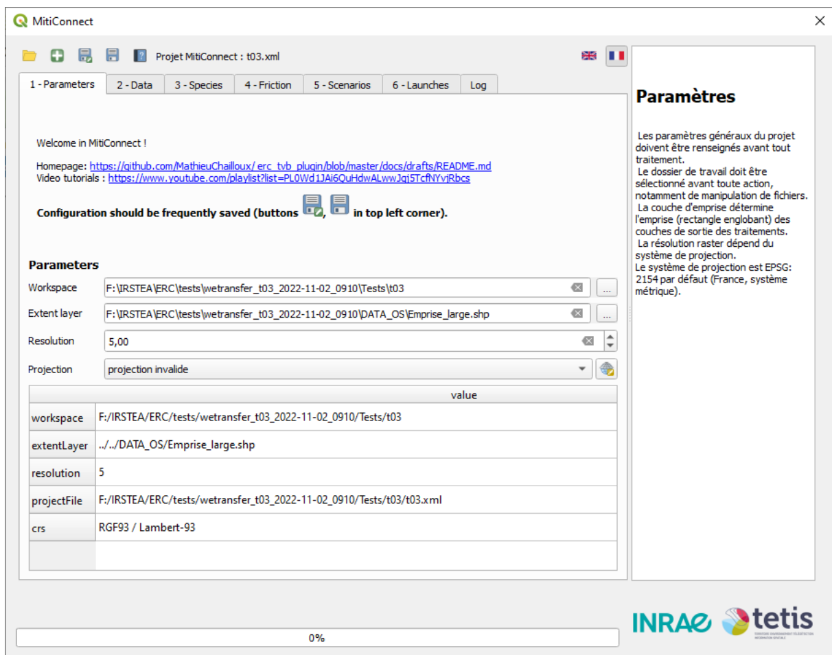
Figure 4: Tab 1 - General settings
